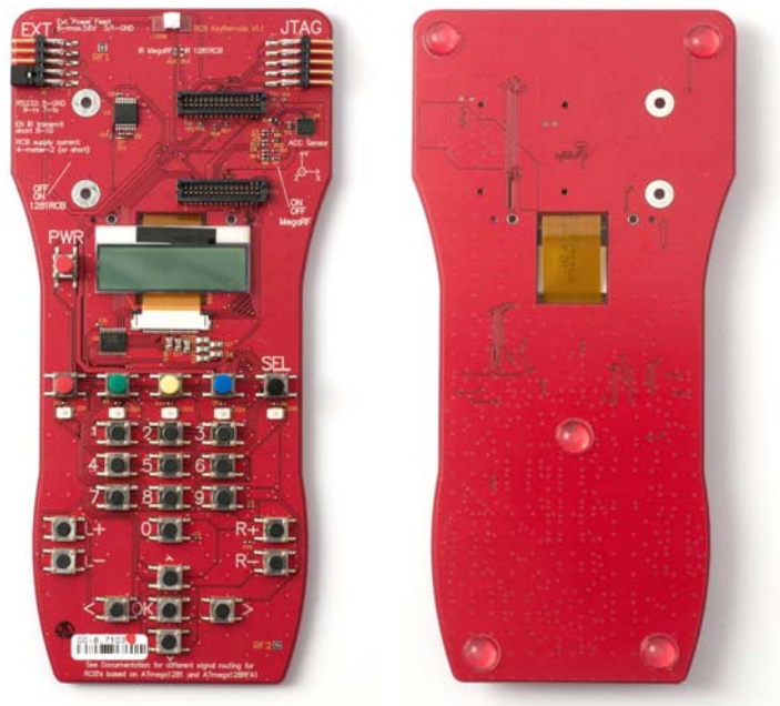
Figure 1-1. RCB Key Remote Control board.
