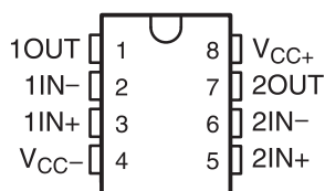
PW PACKAGE TSSOP – 8 (TOP VIEW)
