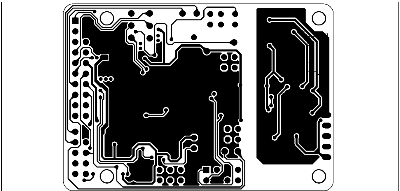
Figure 36 Bottom layer routing of the EVAL-M3-102T
