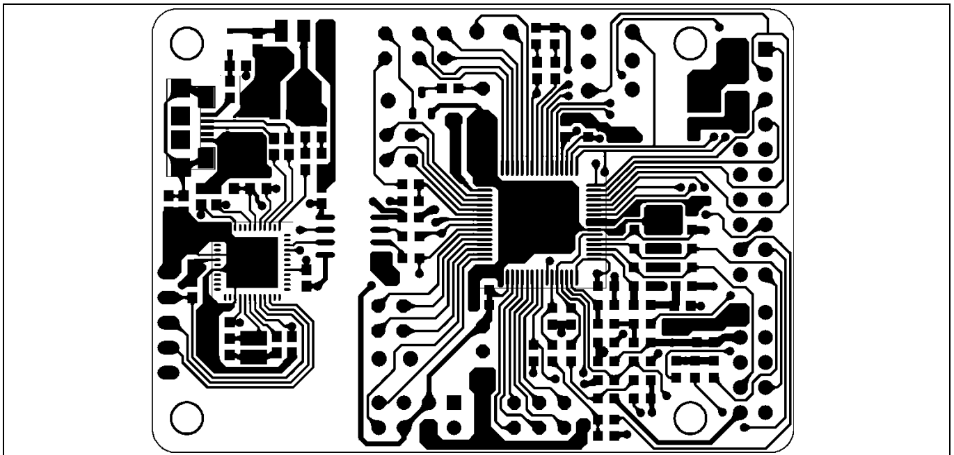
Figure 35 Top layer routing of the EVAL-M3-102T
