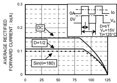
AMBIENT TEMPERATURE : T_a(^{\circ}\text{C}) Derating Curve*( I_o - T_a )
