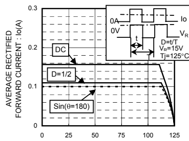
CASE TEMPERATURE : T_c(^{\circ}\text{C}) Derating Curve*( I_o - T_c )
