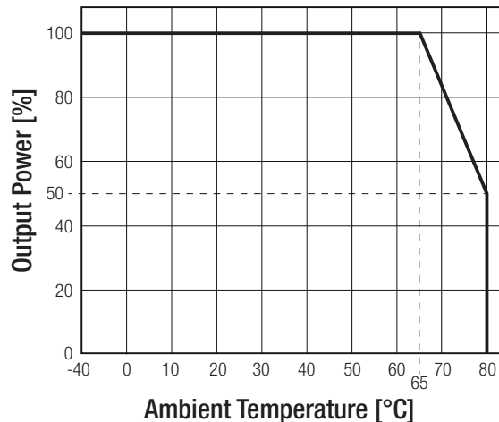
Derating Graph
