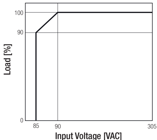
Line Derating (3)
