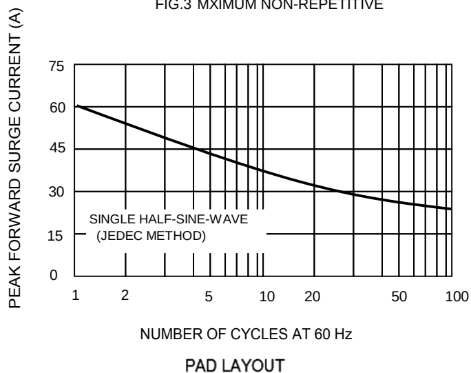
FIG.3 MAXIMUM NON-REPETITIVE
