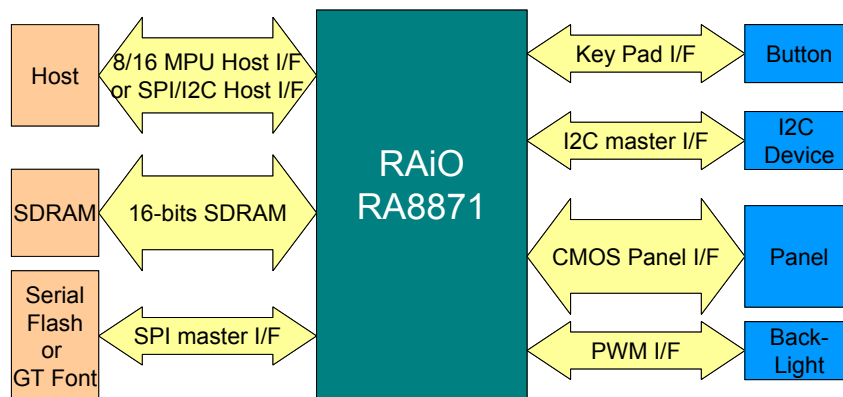
Figure 1-1 : System Diagram
