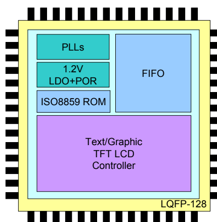
Figure 1-2 : Chip Diagram
