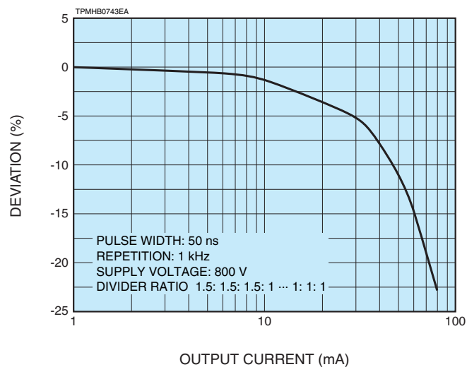
Figure 5: Pulse Linearity (Example)
