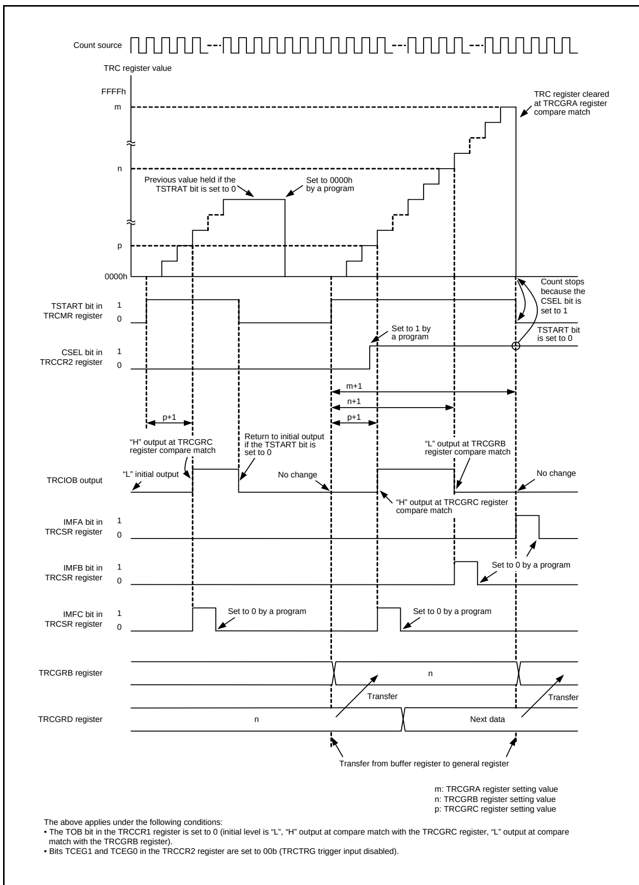
Figure 14.57 Operating Example of PWM2 Mode (TRCTRГ Trigger Input Disabled)
