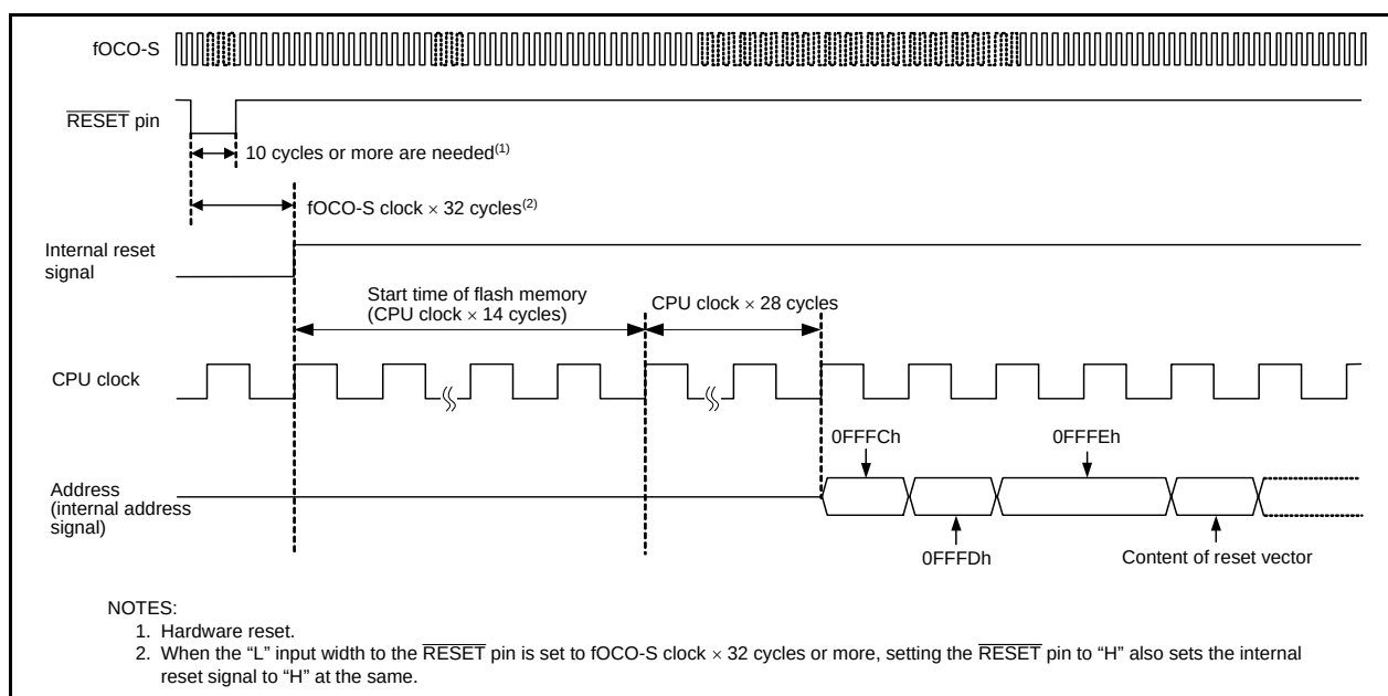
Figure 5.4 Reset Sequence
