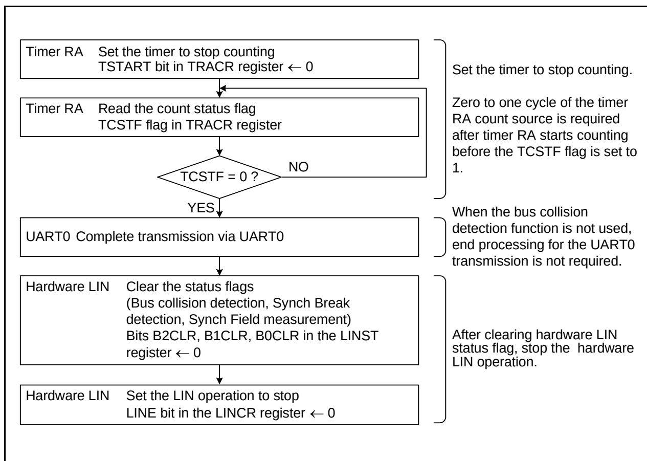
Figure 17.12 Example of Hardware LIN Communication Completion Flowchart
