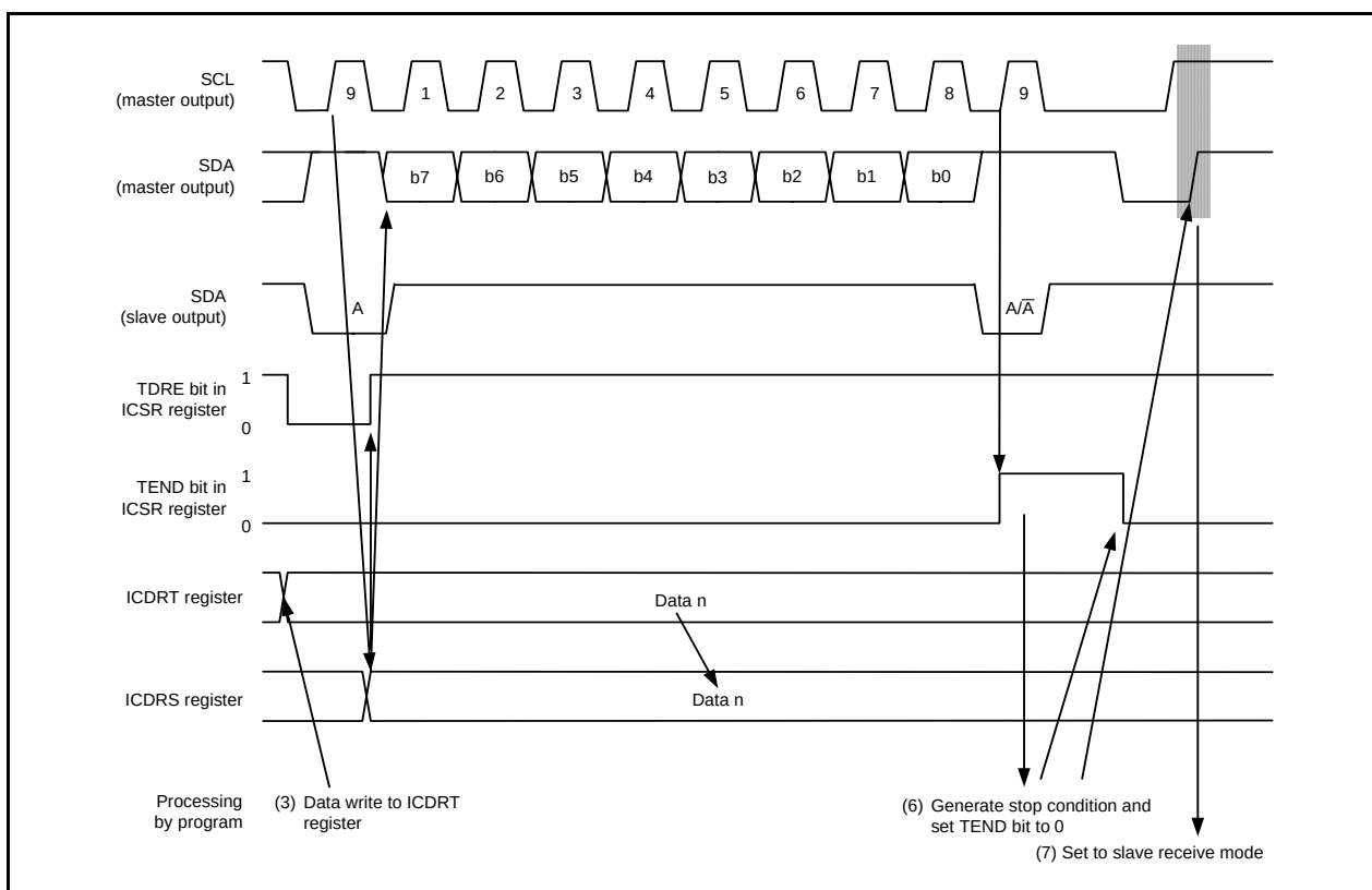
Figure 16.33 Operating Timing in Master Transmit Mode (I²C bus Interface Mode) (2)
