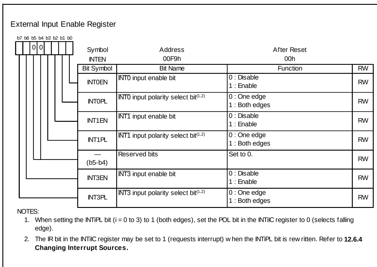
Figure 12.12 INTEN Register
