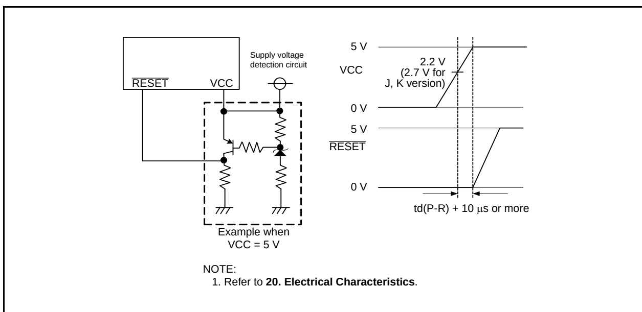
Figure 5.7 Example of Hardware Reset Circuit (Usage Example of External Supply Voltage Detection Circuit) and Operation
