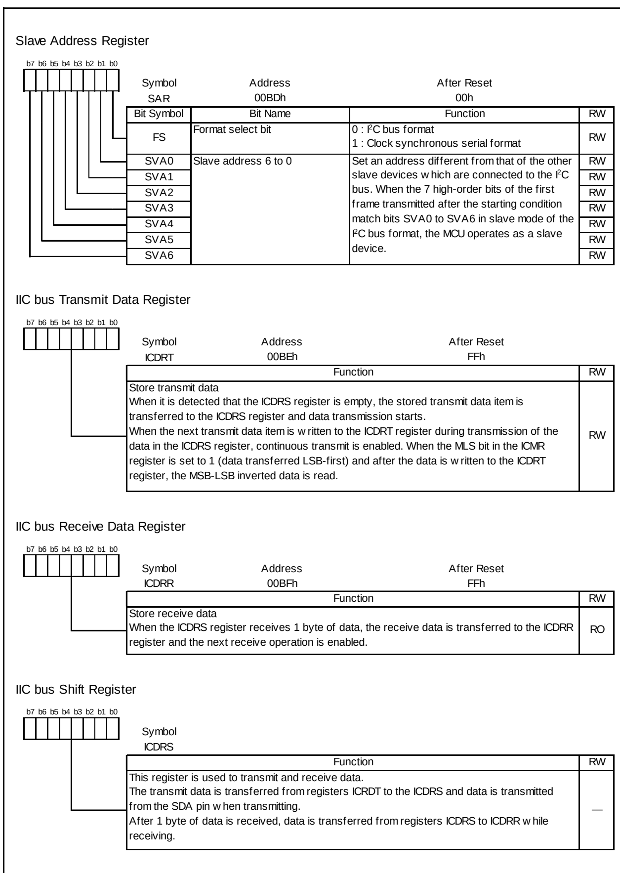
Figure 16.29 Registers SAR, ICDRT, ICDRR, and ICDRS
