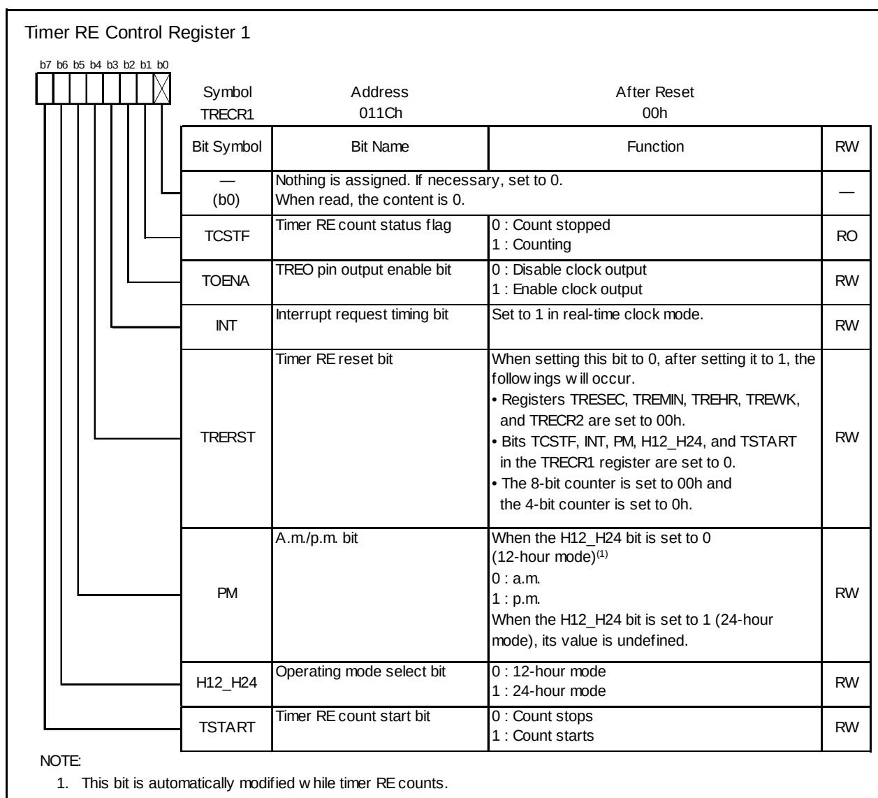
Figure 14.66 TRECRI Register in Real-Time Clock Mode
