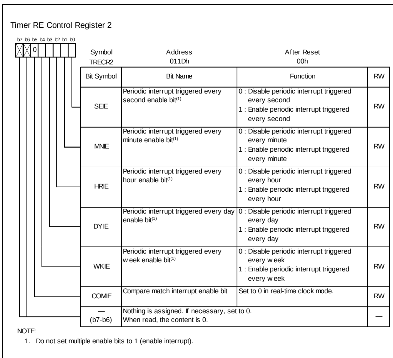
Figure 14.68 TRECR2 Register in Real-Time Clock Mode
