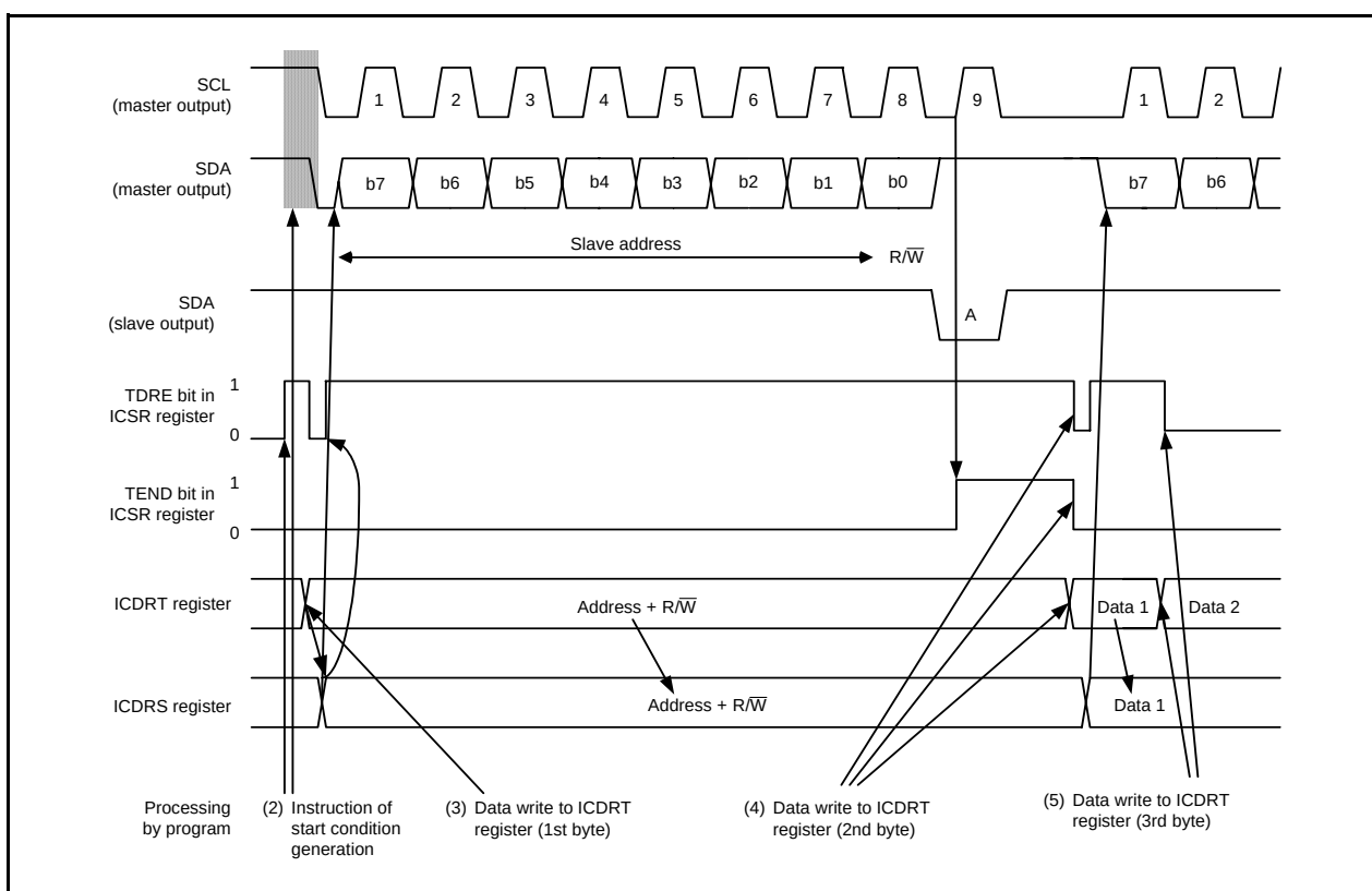
Figure 16.32 Operating Timing in Master Transmit Mode (I²C bus Interface Mode) (1)
