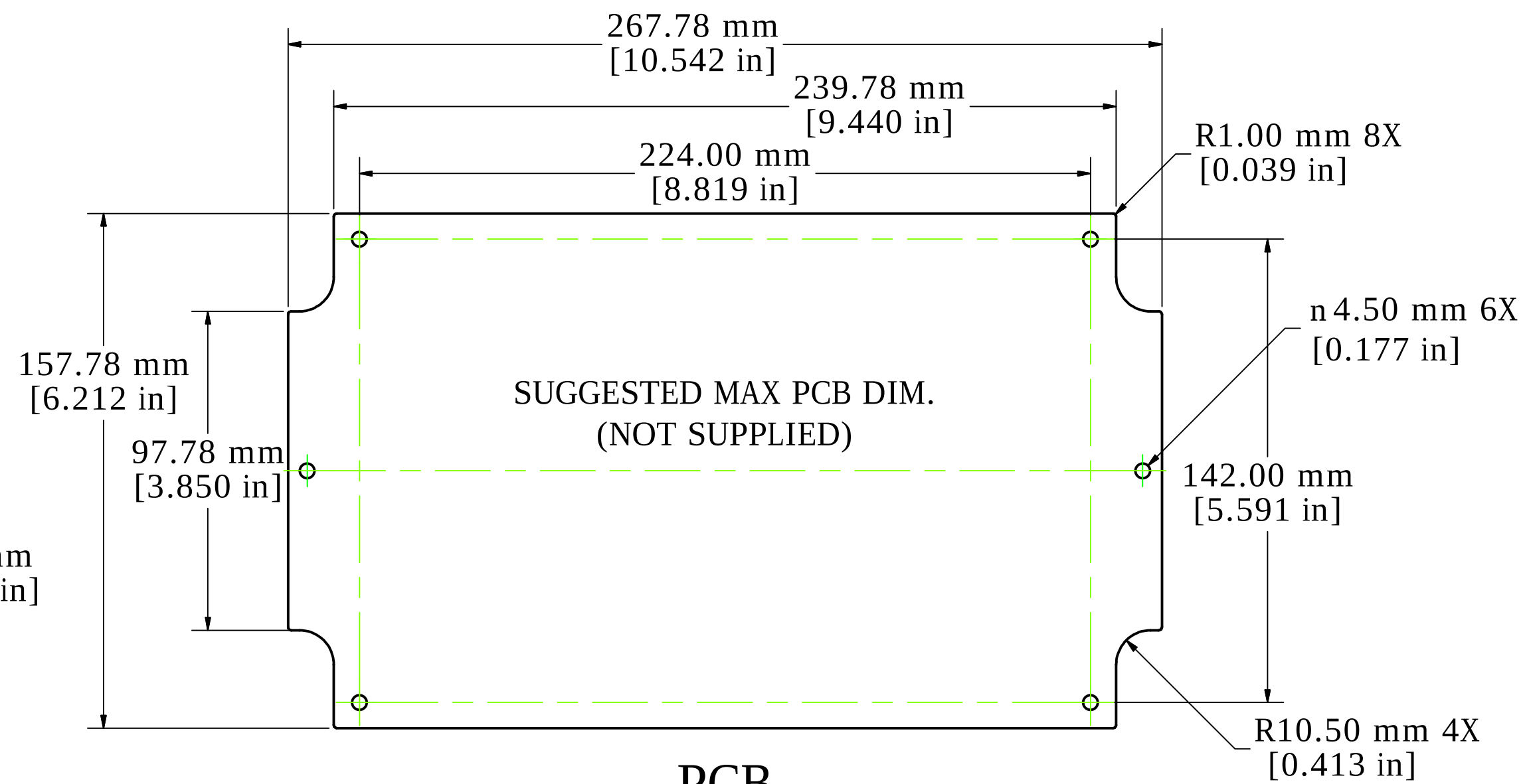
PCB
