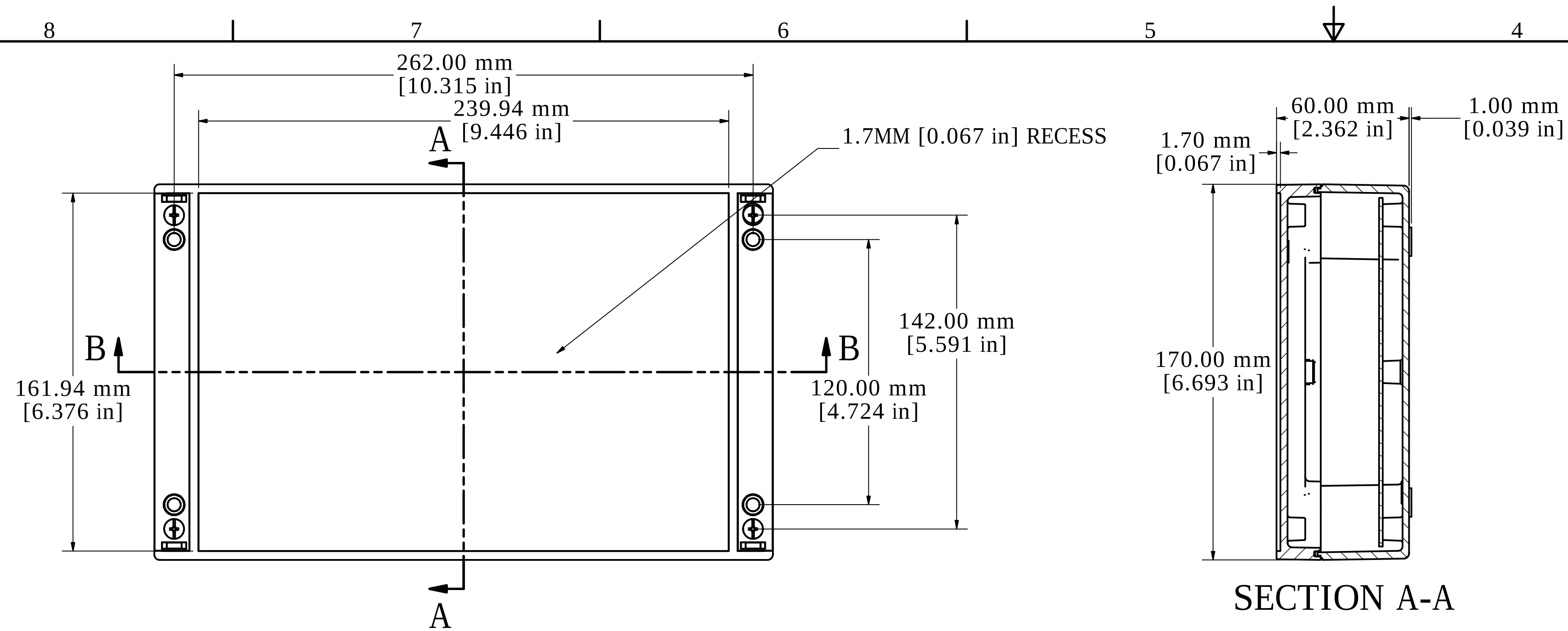
ASSEMBLY - TOP VIEW
