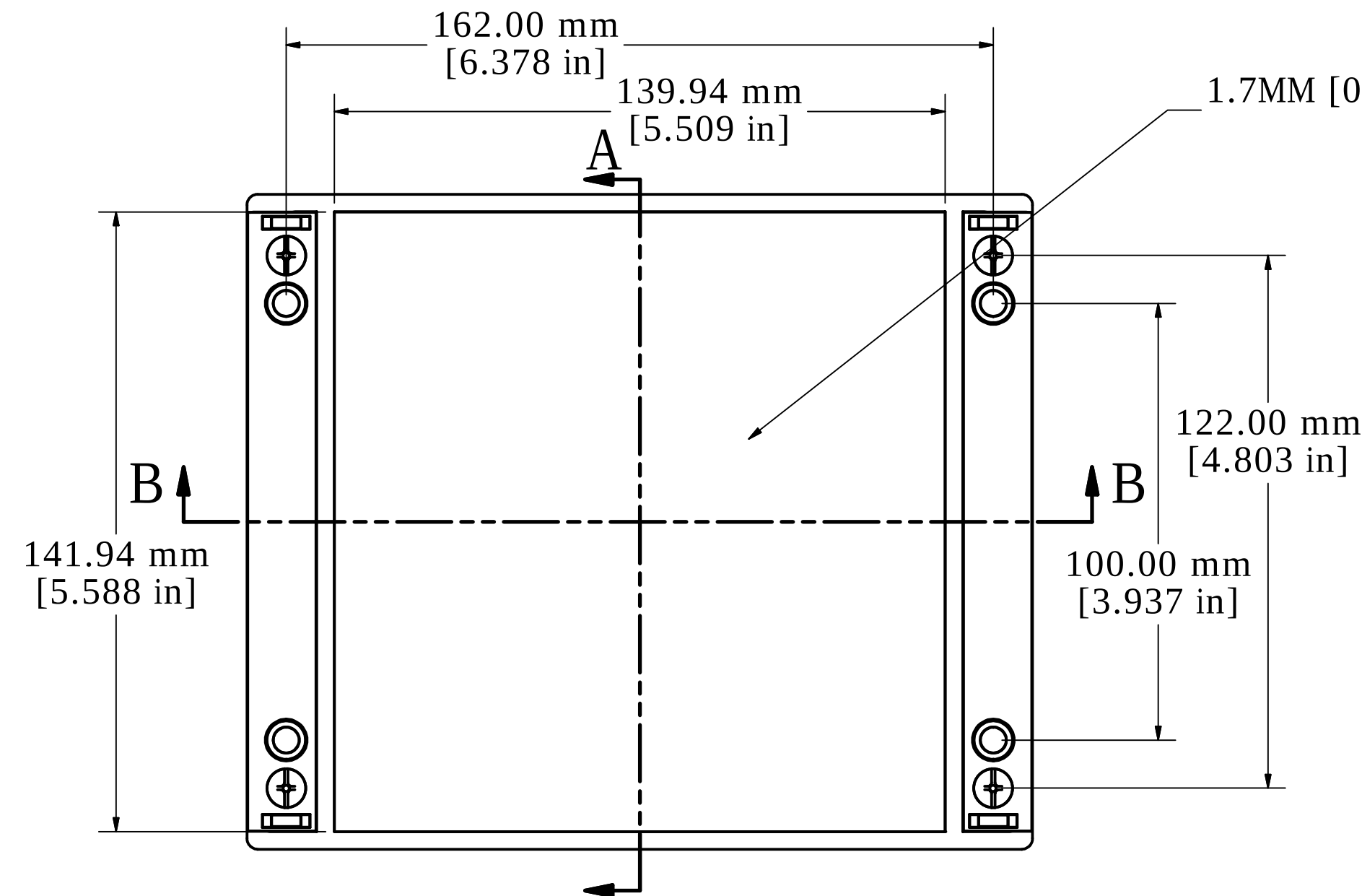
ASSEMBLY - TOP VIEW
