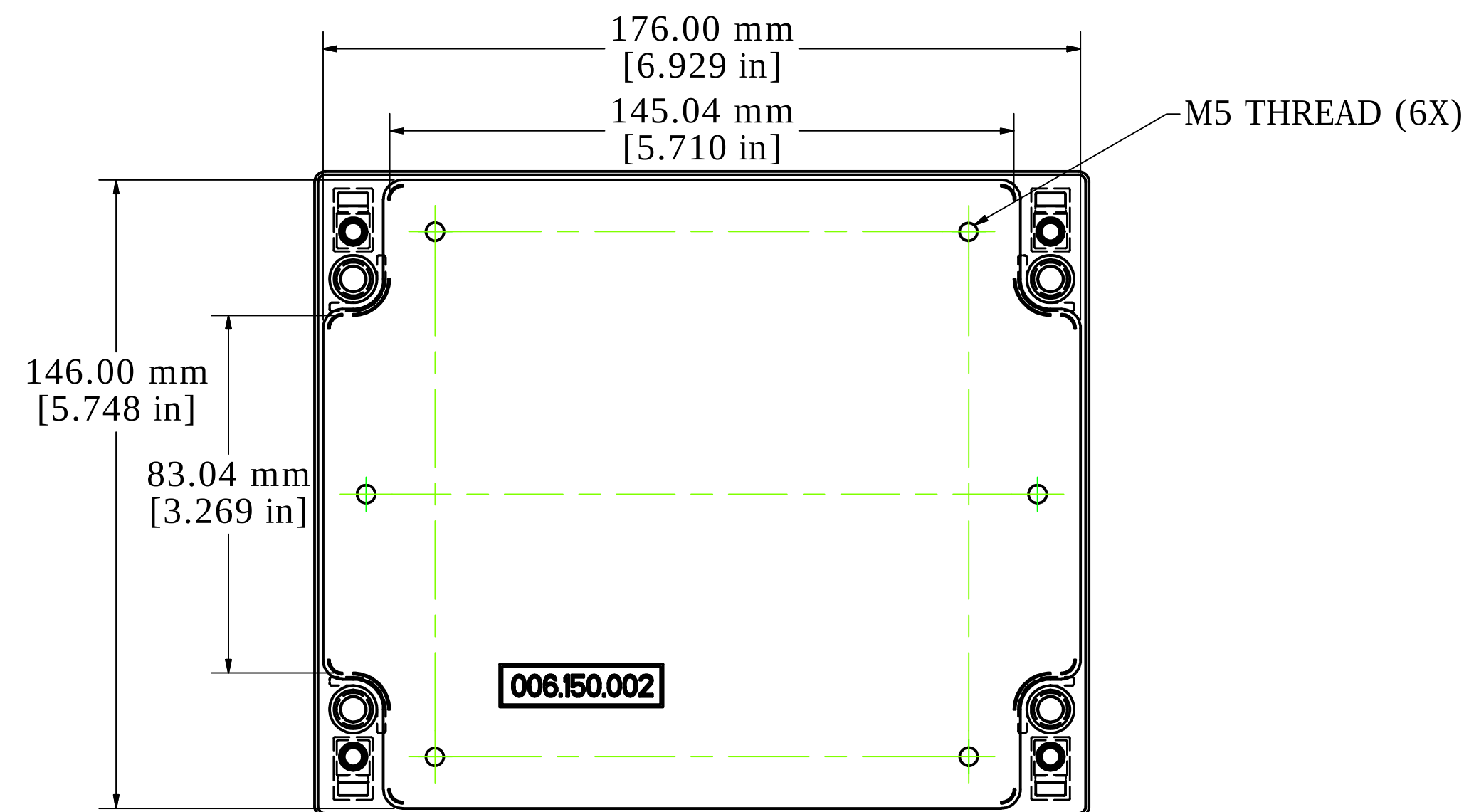
BOX - TOP VIEW
