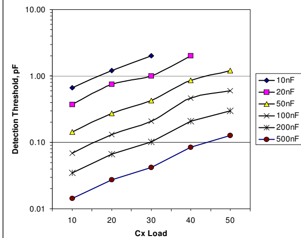
Chart 1 - Threshold Sensitivity vs. Cx, High Gain at Selected Values of Cs
