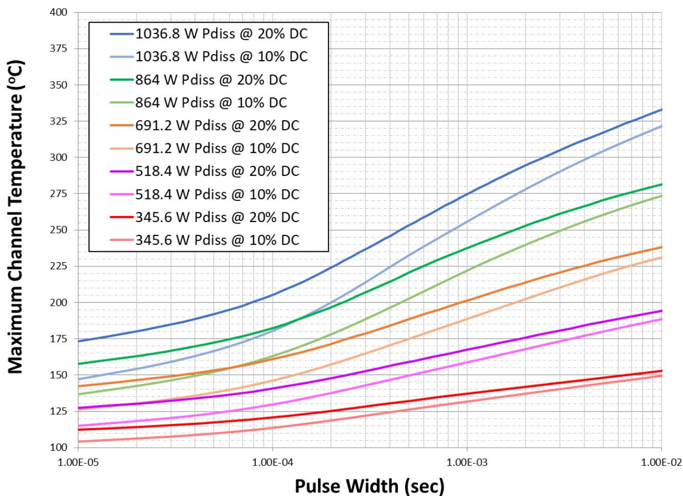
Peak IR Surface Temperature vs. Pulse Width Pallet base fixed at 85 °C, Pdiss Varies
