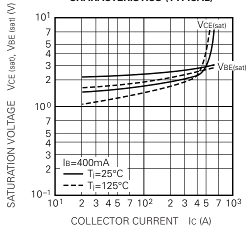
SATURATION VOLTAGE CHARACTERISTICS (TYPICAL)
