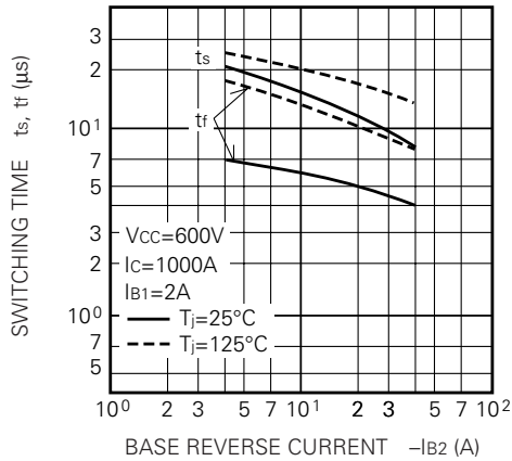
SWITCHING TIME VS. BASE CURRENT (TYPICAL)
