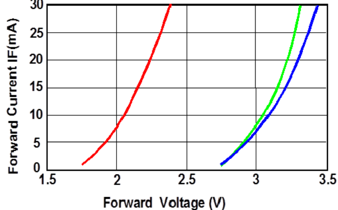
Electrical Characteristics(Ta=25)
