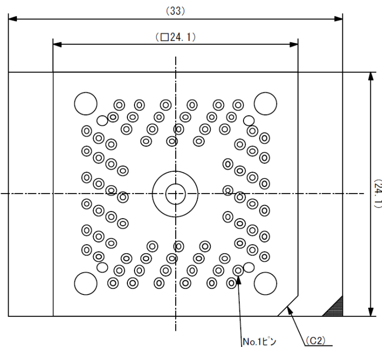
< Bottom view >
