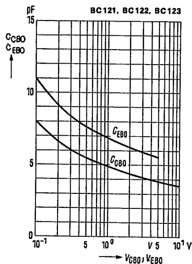
Emitter-base capacitance C_{EB0} = f(V_{EB0}) Collector-base capacitance C_{CB0} = f(V_{CB0})
