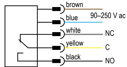
Sensors with Quick-Disconnect 5-Pin Mini-Style (model suffix Q )
