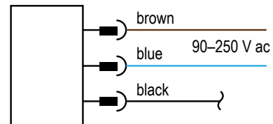
Q452E Emitter with Quick-Disconnect 3-Pin Mini-Style (model suffix Q )
