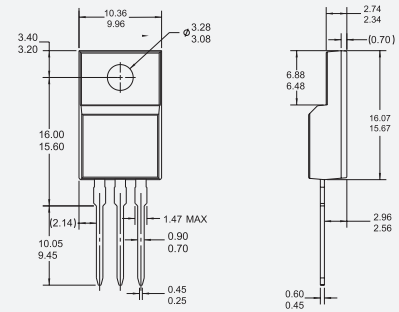
TO-220 [KF]
