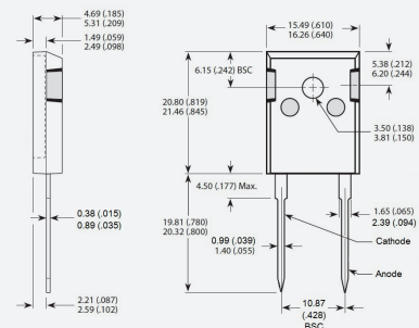
TO-247 2-Lead
