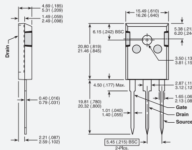
TO-247 3-Lead
