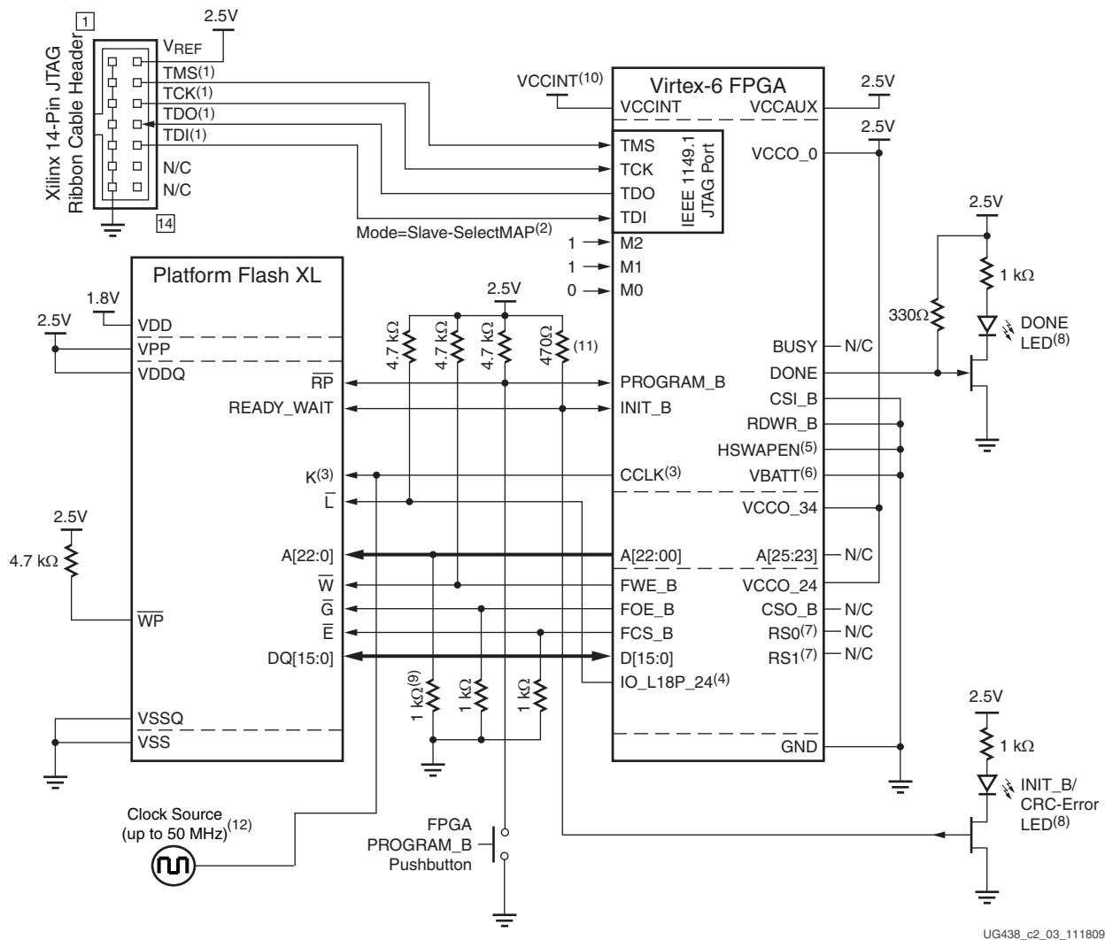
Figure 2-2: Virtex-6 FPGA Slave SelectMAP Configuration Mode from Platform Flash XL
