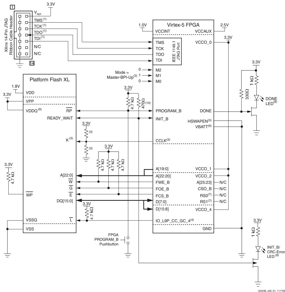
Figure 3-1: Virtex-5 FPGA Master BPI-Up Configuration Mode from Platform Flash XL with Indirect Programming Support
