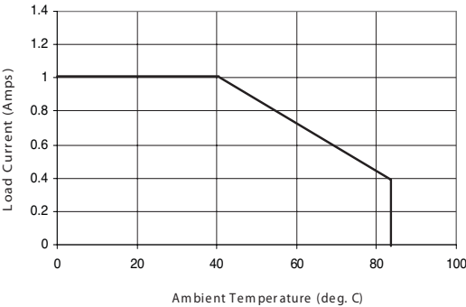
Figure 1. Current Derating Curves
