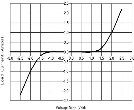
Figure 3. Output Characteristics
