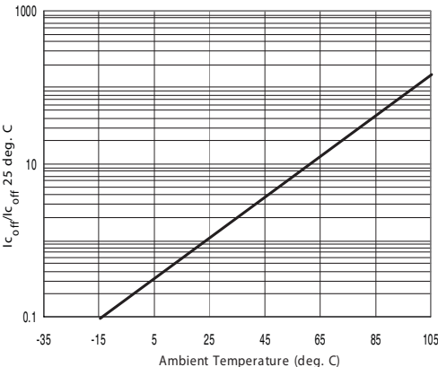
Figure 5. Typical Normalized Off-State Leakage
