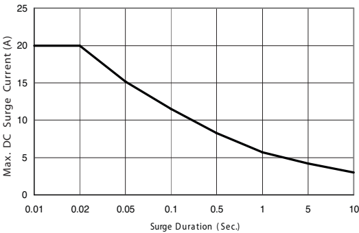
Figure 2. Surge Current Capability
