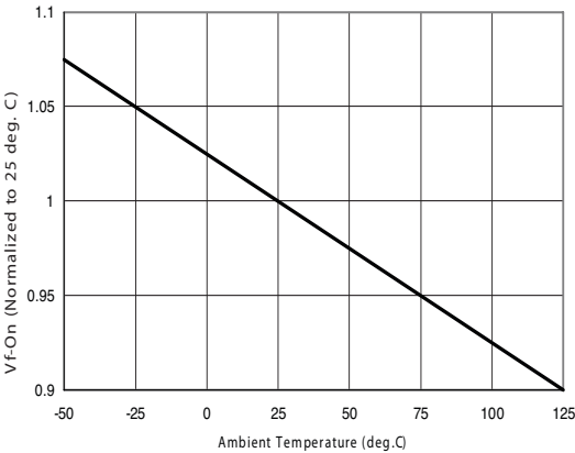
Figure 4. Typical Normalized V_{CEON}
