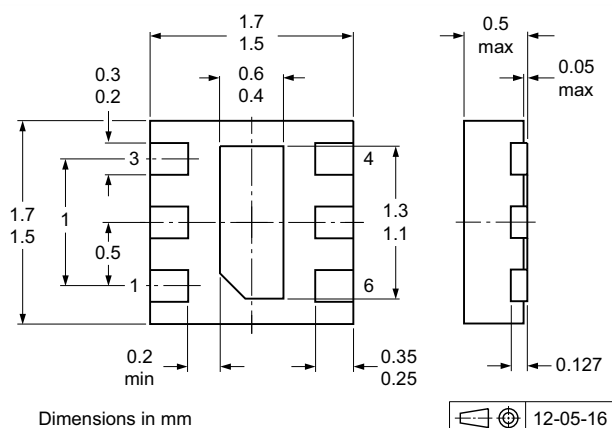
Fig 4. Package outline DFN1616-6 (SOT1189-1/XSON6)
