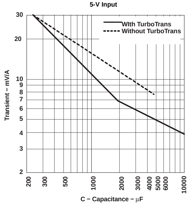
Figure 17. Cap Type C, 5000 < C(\mu F) \times ESR(m\Omega) \leq 10,000 (e.g. OS-CON)
