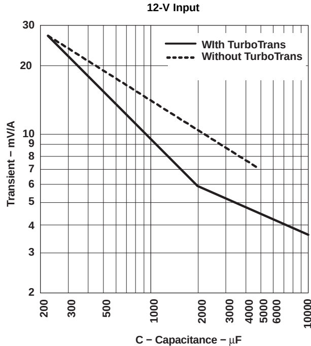
Figure 16. Cap Type C, 5000 < C(\mu F) \times ESR(m\Omega) \leq 10,000 (e.g. OS-CON)
