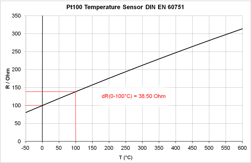
Figure 1: Resistance characteristics
