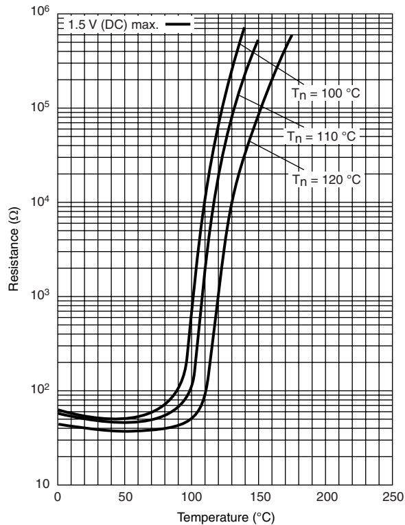
TYPICAL RESISTANCE/TEMPERATURE CHARACTERISTIC FOR 2381 671 91109
