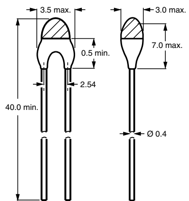
Component outline for 91152 to 91164
