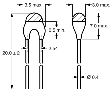
Component outline for 91102 to 91114
