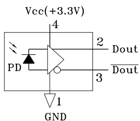
TYPE A
