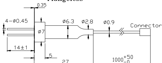
Vertical Flange
