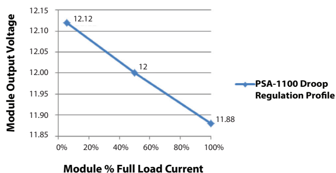
PSA-1100 Droop Regulation Profile
