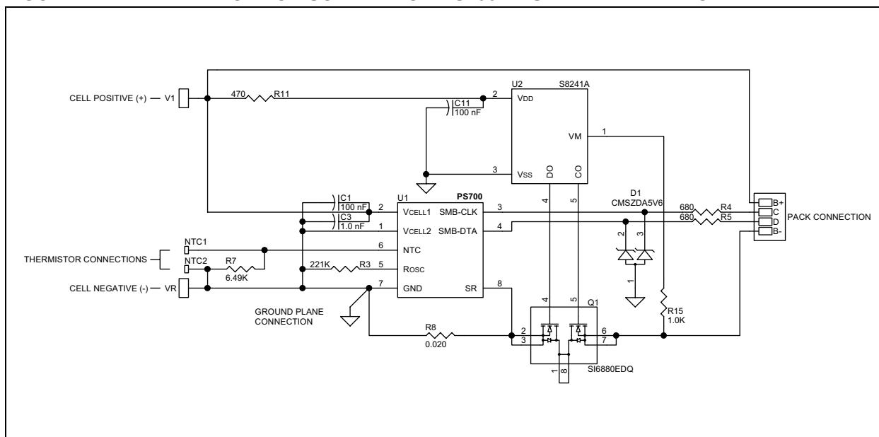
FIGURE 1-2: APPLICATION SCHEMATIC – PS700-BASED BATTERY PACK
