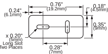
Option with Slit: Modify Beam Size of Through-Beam Sensor
