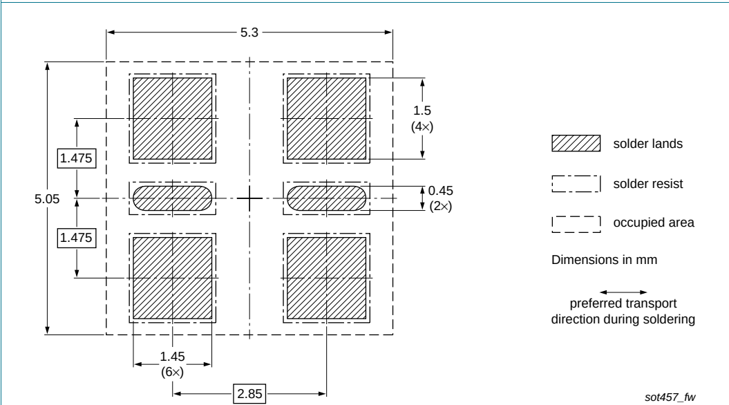
Fig 5. Wave soldering footprint SOT457 (SC-74)
