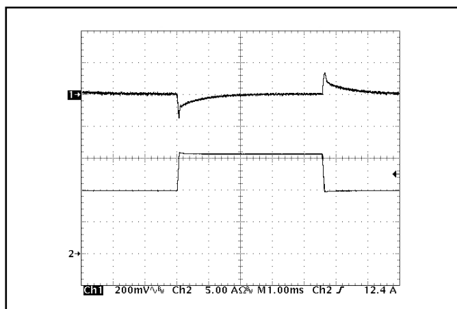
Figure 15: Output voltage response to step-change in load current (50%-75%-50% of I_{out(max)} ; dI/dt = 0.1A/\mu s ). Load cap: 10 \mu F , 100 m \Omega ESR tantalum capacitor and 1 \mu F ceramic capacitor. Ch 1: Vout (200mV/div), Ch 2: Iout (5A/div).
