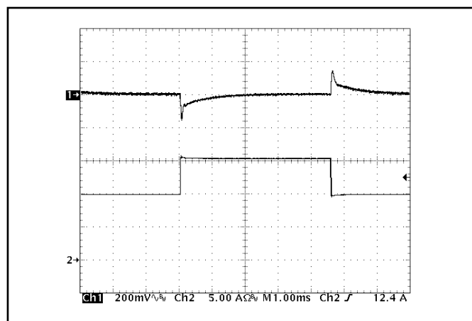
Figure 16: Output voltage response to step-change in load current (50%-75%-50% of I_{out(max)} ; dI/dt = 5A/\mu s ). Load cap: 470 \mu F , 30 m \Omega ESR tantalum capacitor and 1 \mu F ceramic cap. Ch 1: Vout (200mV/div), Ch 2: Iout (5A/div).
