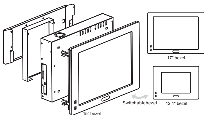
12.1" / 15" / 17" Modularizing View
