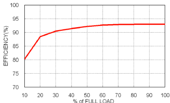
POL10-12T, Vout=3.3V Efficiency vs. Output Load
