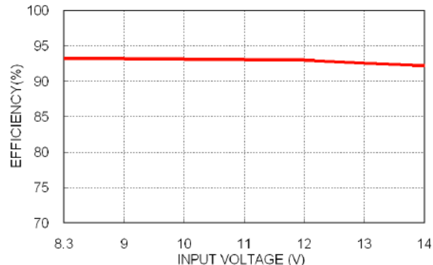
POL10-12T, Vout=3.3V Efficiency vs. Input Voltage
