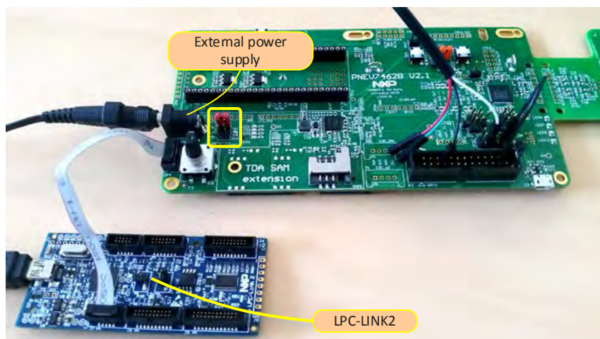
Fig 6. LPC Link2 connection for debugging and flashing
