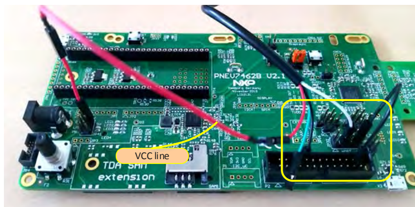
Fig 5. USB powered setup (setup without any external power supply)
