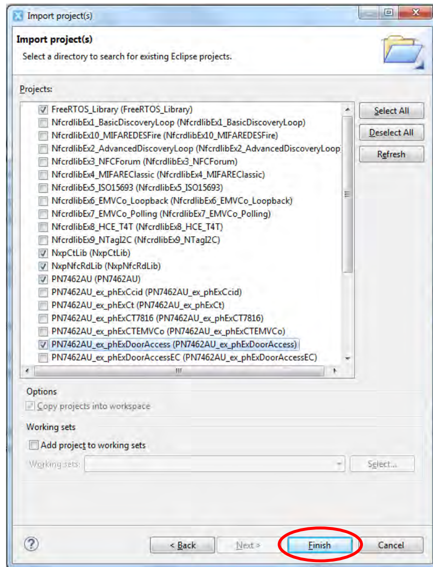
Fig 9. Select project
