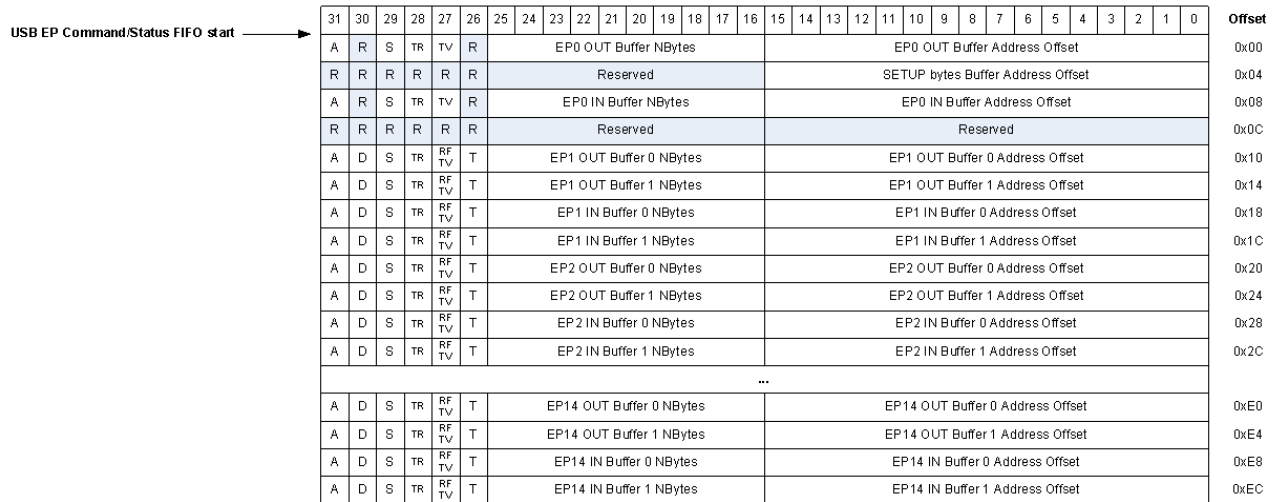
Fig 69. Endpoint command/status list
