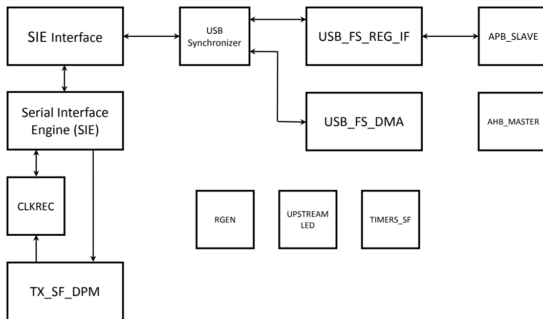
Fig 67. USB block diagram
