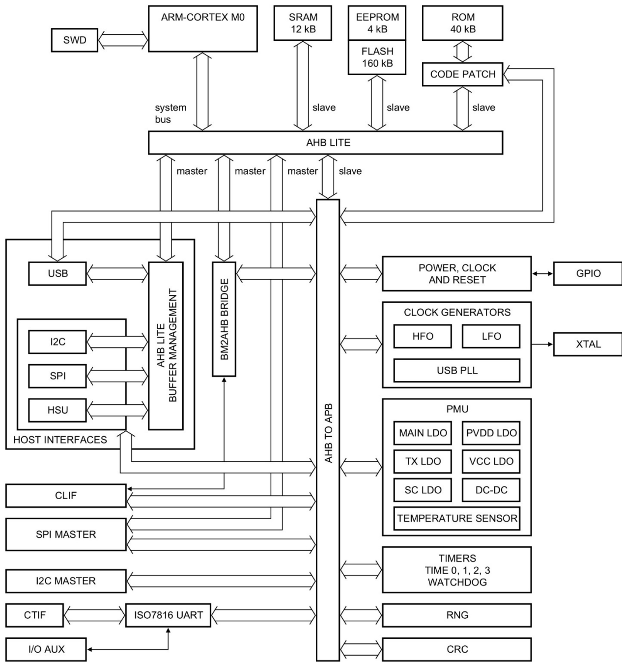
Fig 1. Block diagram
