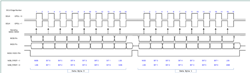
Fig 51. SPI protocol with CPHA = 0 & NSS_PULSE = 1
