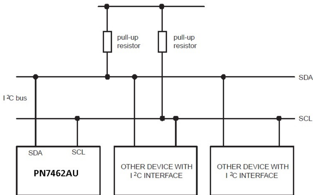
Fig 42. I 2 C bus configuration
