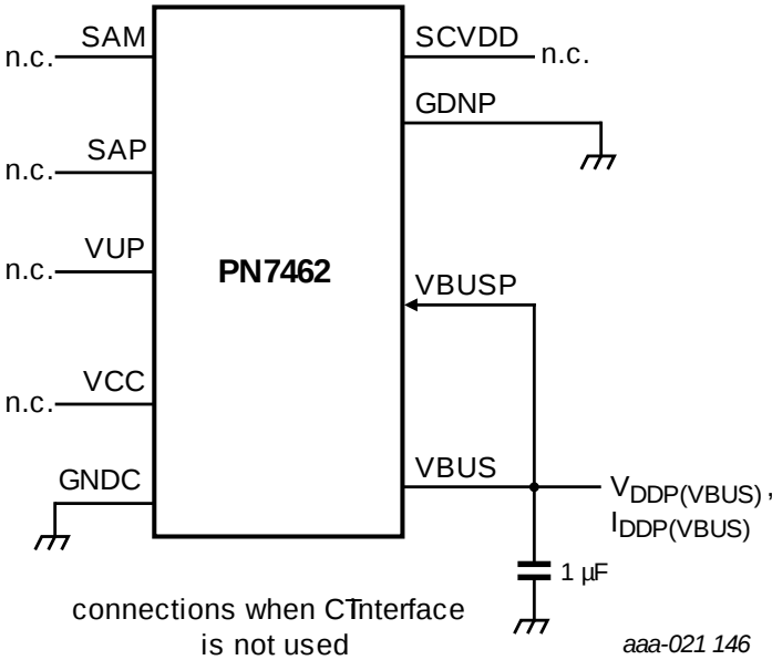
Fig 14. Contact interface power supply connection when the contact interface is not used
