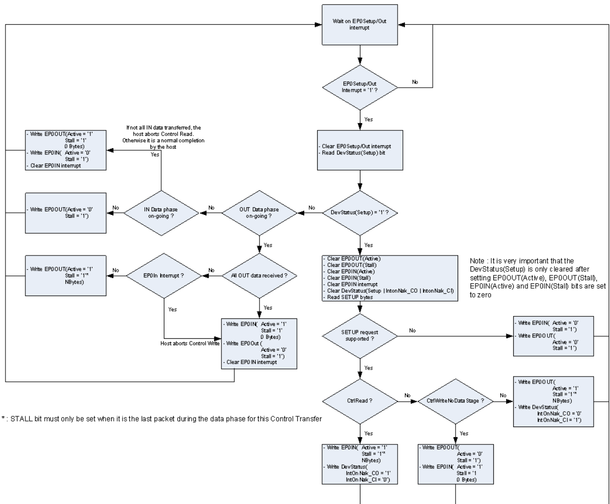
Fig 70. Control endpoint zero – OUT direction
