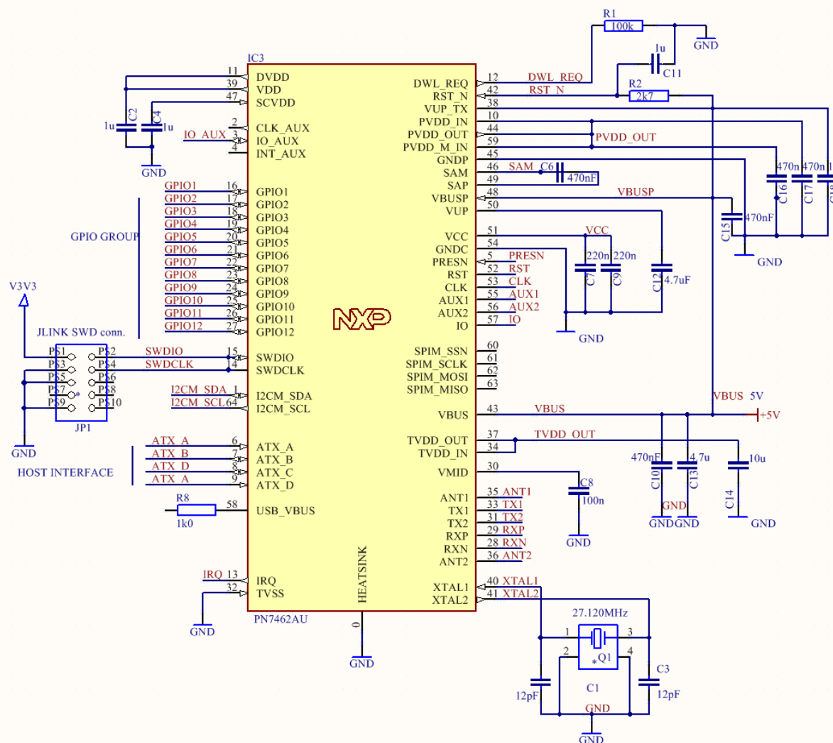
Fig 16. PN7462 family basic schematic
