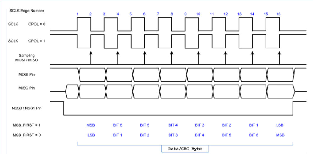
Fig 50. SPI protocol with CPHA = 1 & NSS_PULSE = 0
