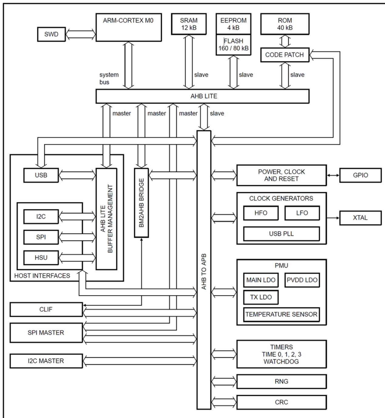
Fig 3. Block diagram
