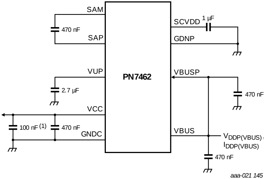
Fig 13. Powering the contact interface
