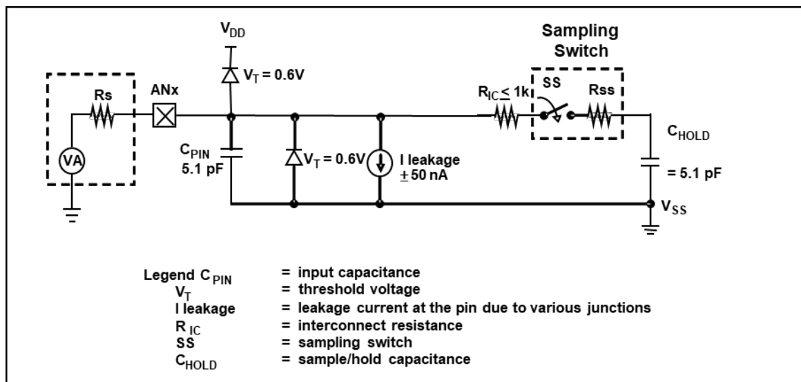
Fig.13: Analog Input Model
