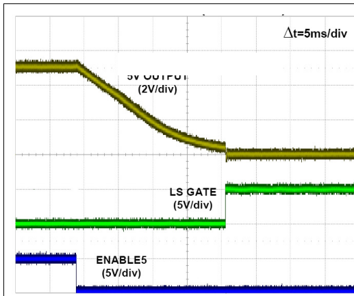
Figure 23. 5V soft end (1Ω load)
