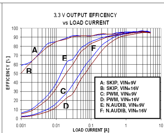
Figure 4. 3.3V output efficiency vs load current
