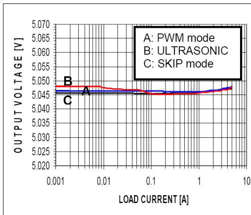
Figure 13. 5V voltage regulation vs load current
