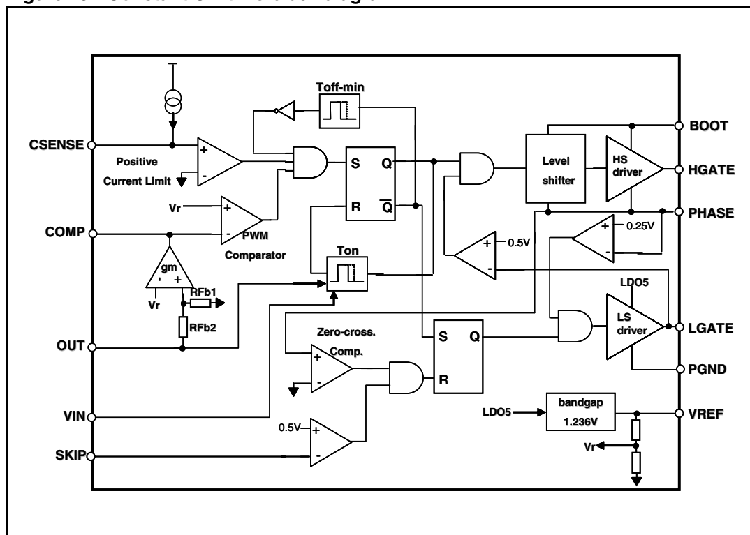
Figure 29. Constant ON-time block diagram
