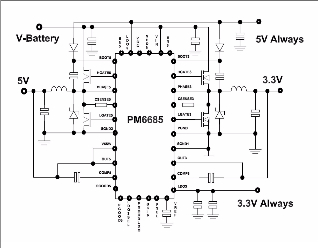
Figure 1. Circuit
