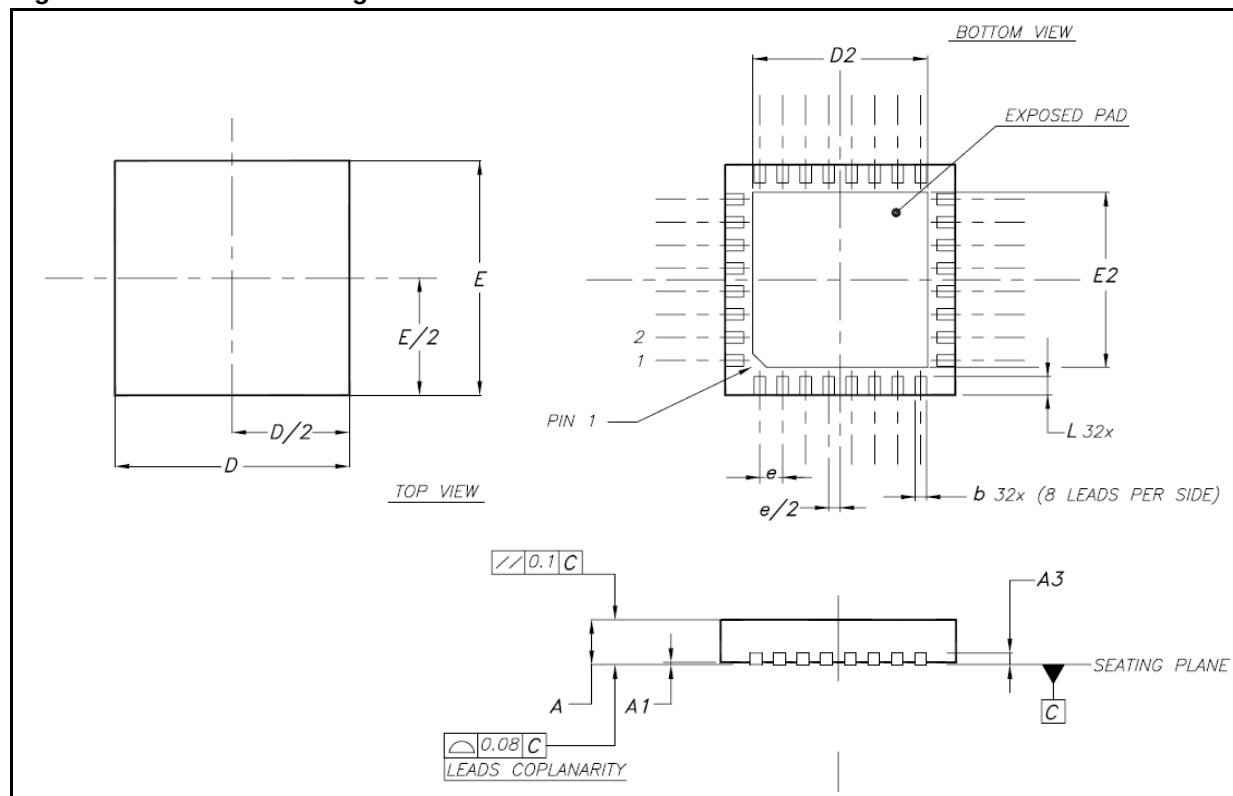
Figure 4. Scheme Drawings
