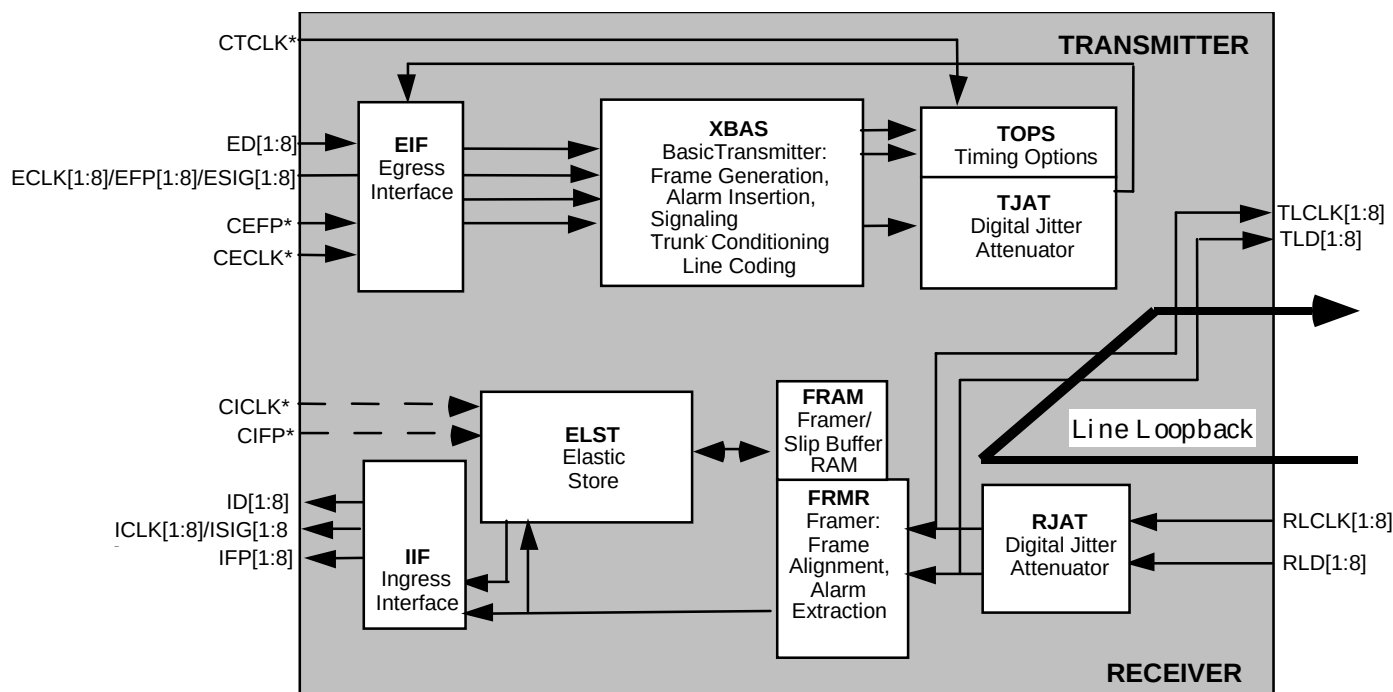
Figure 27 - Line Loopback
