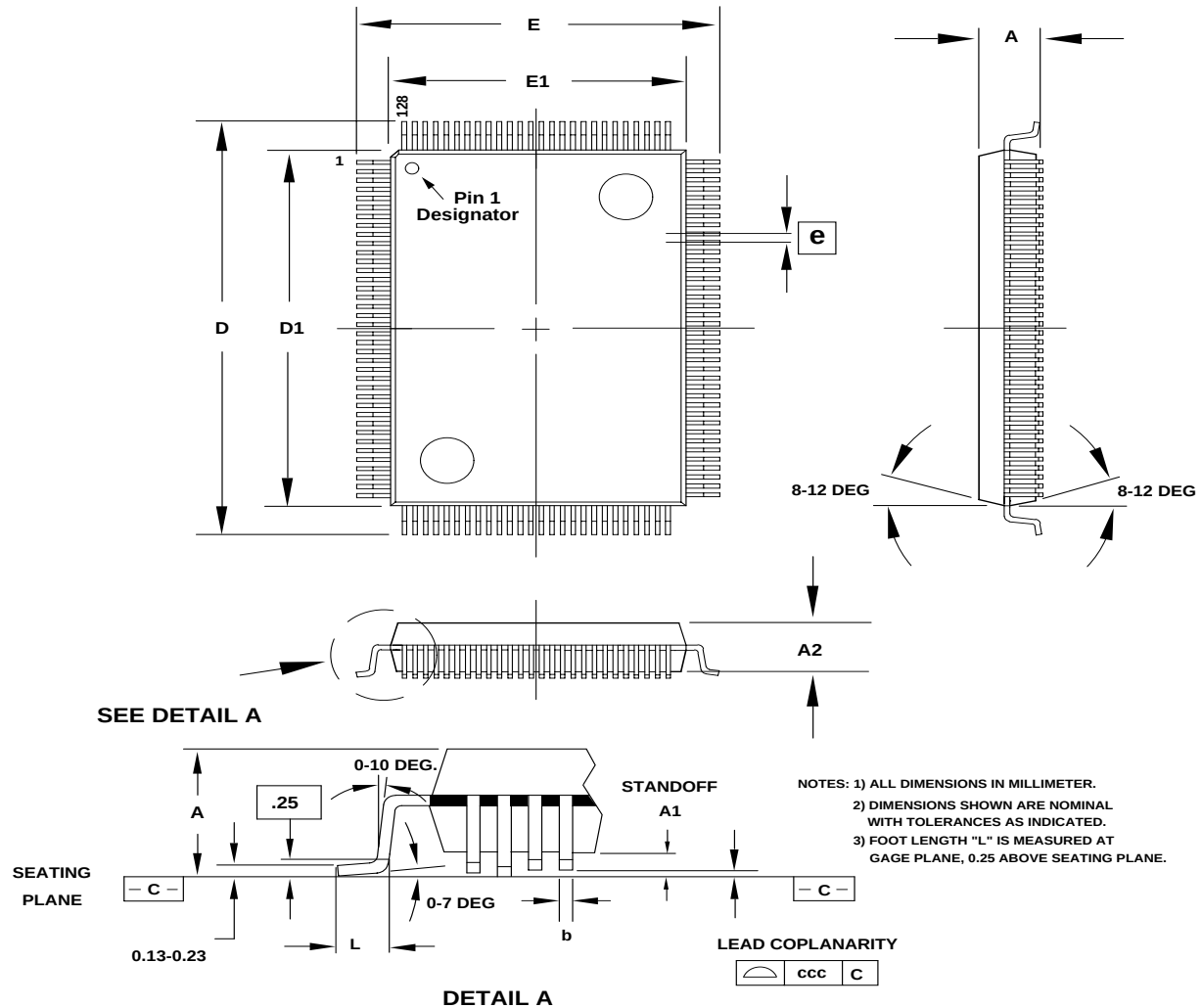
Figure 49 - 128 Pin Copper Leadframe Plastic Quad Flat Pack (R Suffix):
