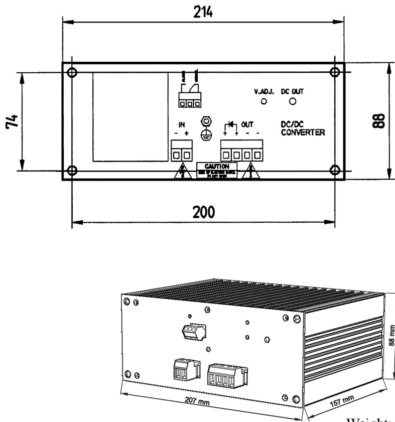
Figure 1. Dimensions Weight: 2.5 l
