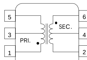
SCHEMATIC "G"
