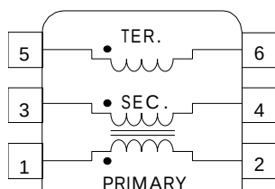
SCHEMATIC "A"
