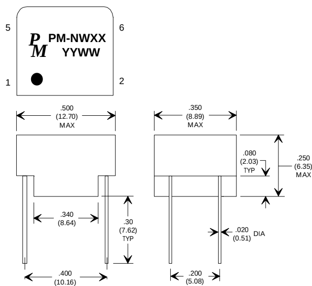
Schematic "B" Pin #3 & 6 Removed
