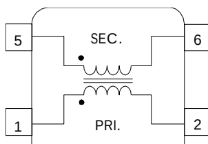
SCHEMATIC "B"
