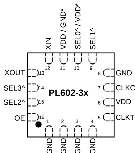
QFN-16L
