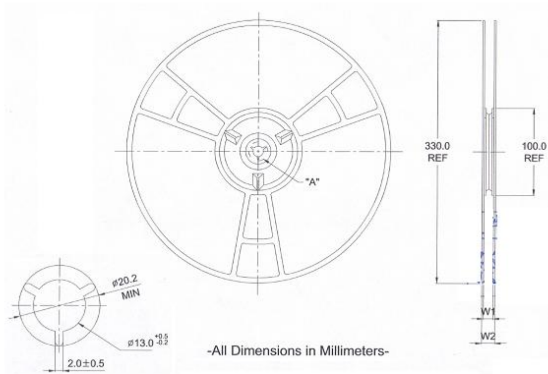
Figure 11-4 Reel Dimension
