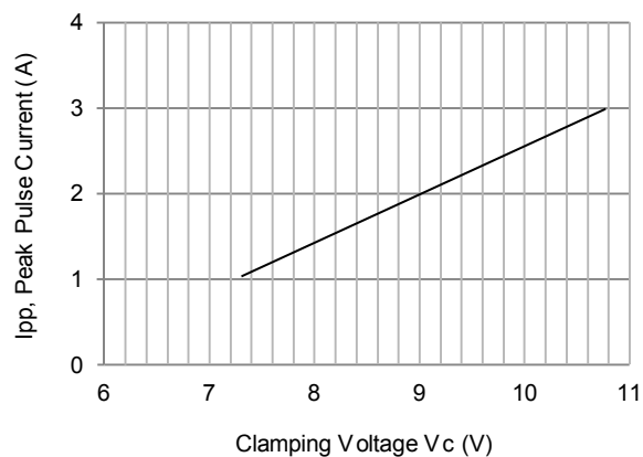
Typical Peak Clamping Voltage (8/20 \mu S)
