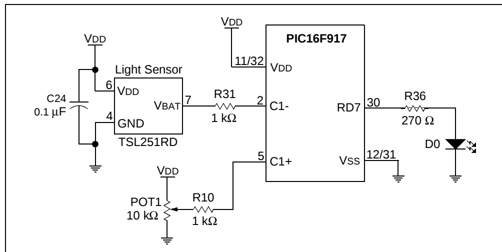
FIGURE 2-5: PROJECT 2: SCHEMATIC
