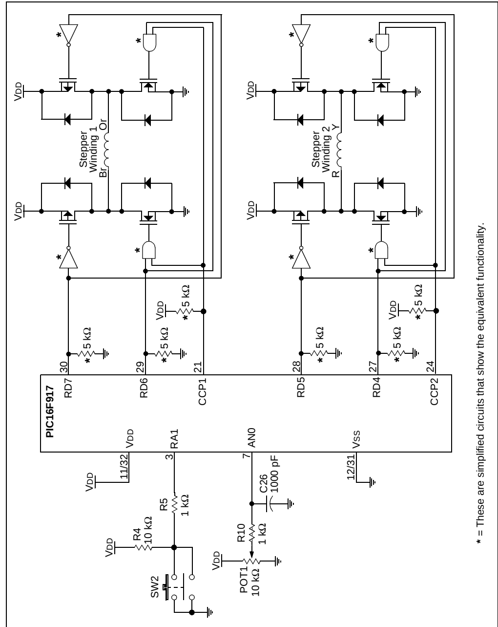
FIGURE 2-15: PROJECT 7: SCHEMATIC
