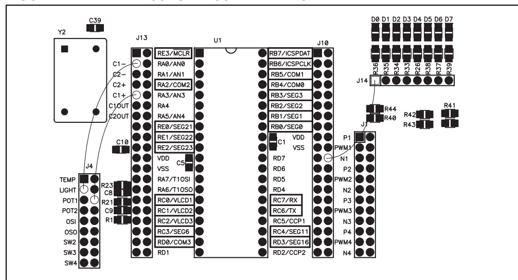
FIGURE 2-4: PROJECT 2: JUMPER DIAGRAM
