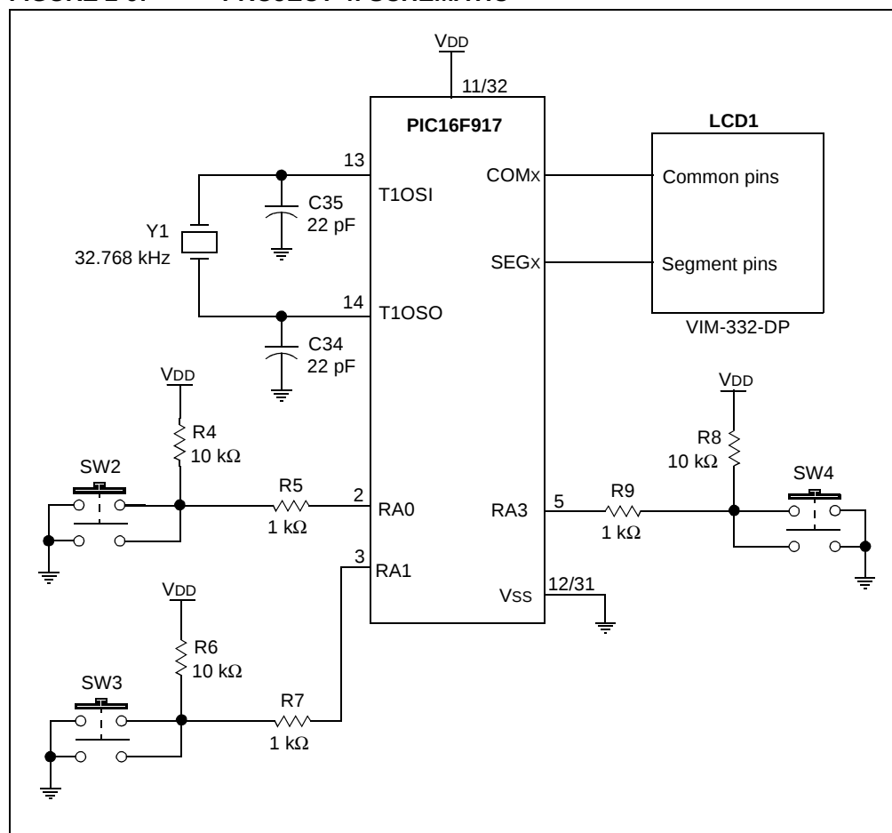
FIGURE 2-9: PROJECT 4: SCHEMATIC
