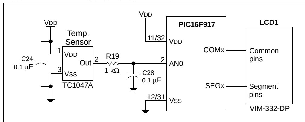
FIGURE 2-7: PROJECT 3: SCHEMATIC
