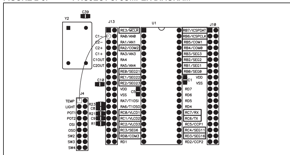
FIGURE 2-6: PROJECT 3: JUMPER DIAGRAM
