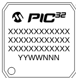
144-Lead TQFP (16x16x1 mm)
