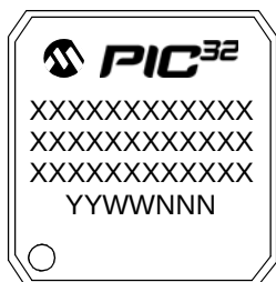
144-Lead LQFP (20x20x1.40 mm)
