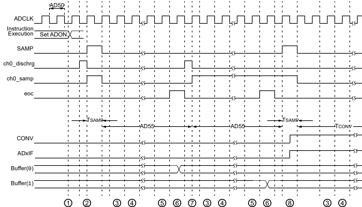
FIGURE 33-19: ANALOG-TO-DIGITAL CONVERSION (10-BIT MODE) TIMING CHARACTERISTICS (ASAM = 1, SSRC<2:0> = 111, SAMC<4:0> = 00001)
