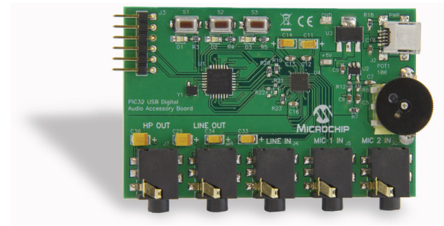
FIGURE 1: PIC32 USB DIGITAL AUDIO ACCESSORY BOARD
