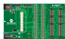
I/O Expansion Board (DM320002)
